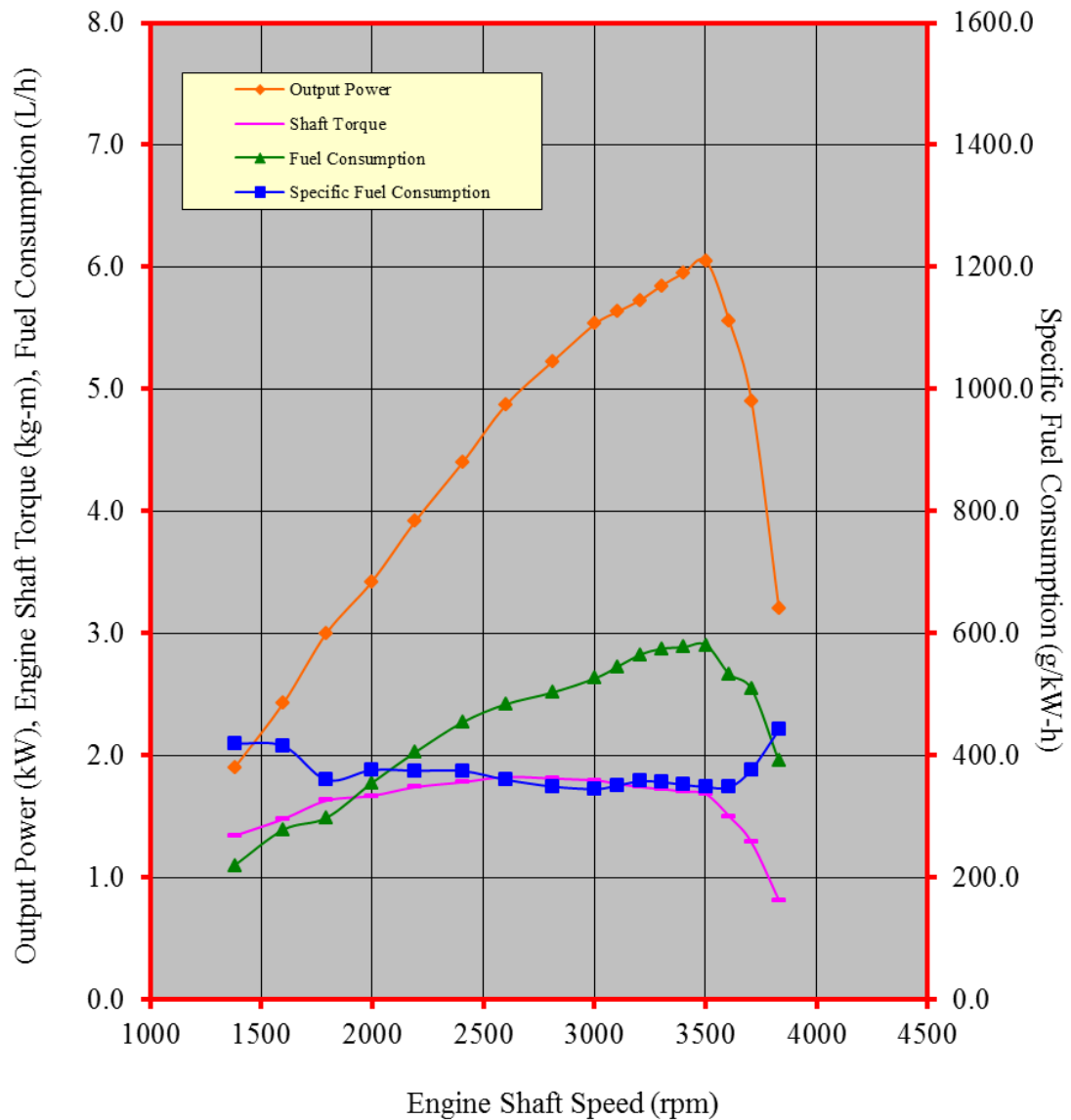
Figure 2. Performance characteristic curves of the HONDA GX270 gasoline engine (using dry dual type air cleaner)
