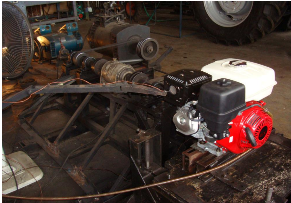
Figure 2. Test set-up of the HONDA GX270 Gasoline Engine (using dry dual type air cleaner).
