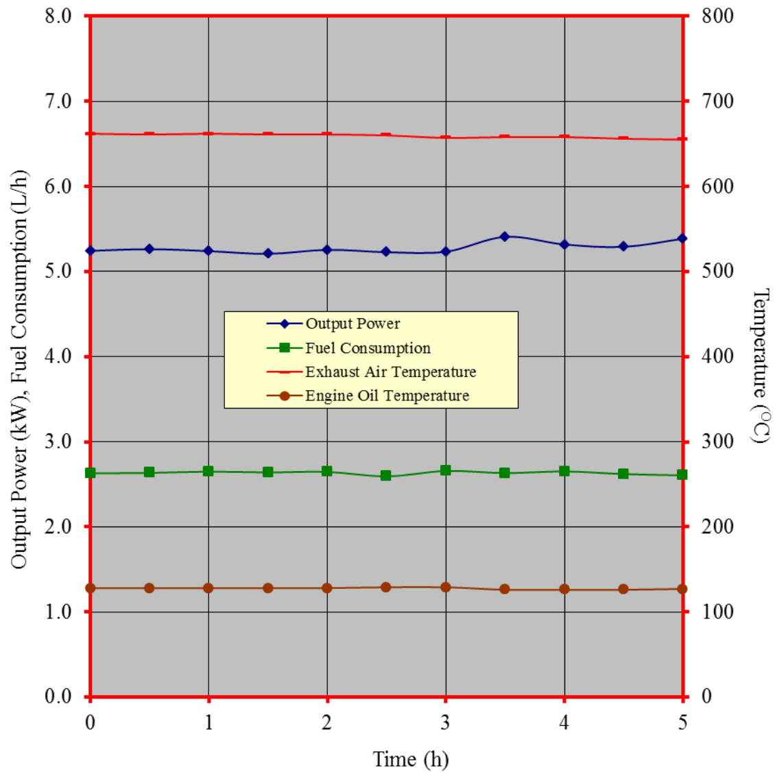
Figure 3. Performance characteristic curves during the continuous running test of the HONDA GX270 gasoline engine (using dry dual type air cleaner)
